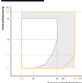
Warm tapwater
